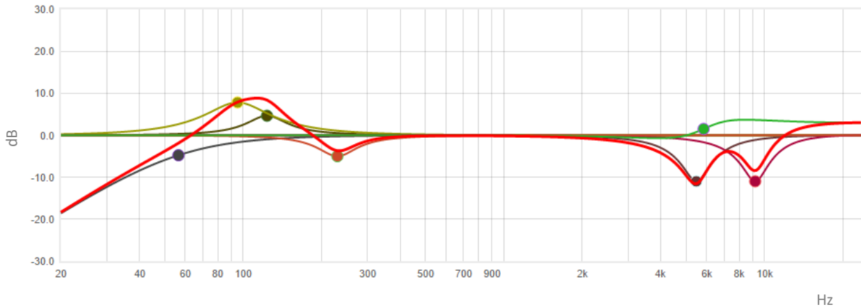
Equalization Curve – single Frequency Points
