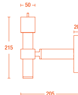
Wall bracket
