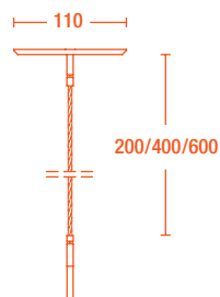
Ceiling mount assembly
