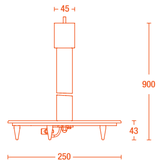
Floor stand
